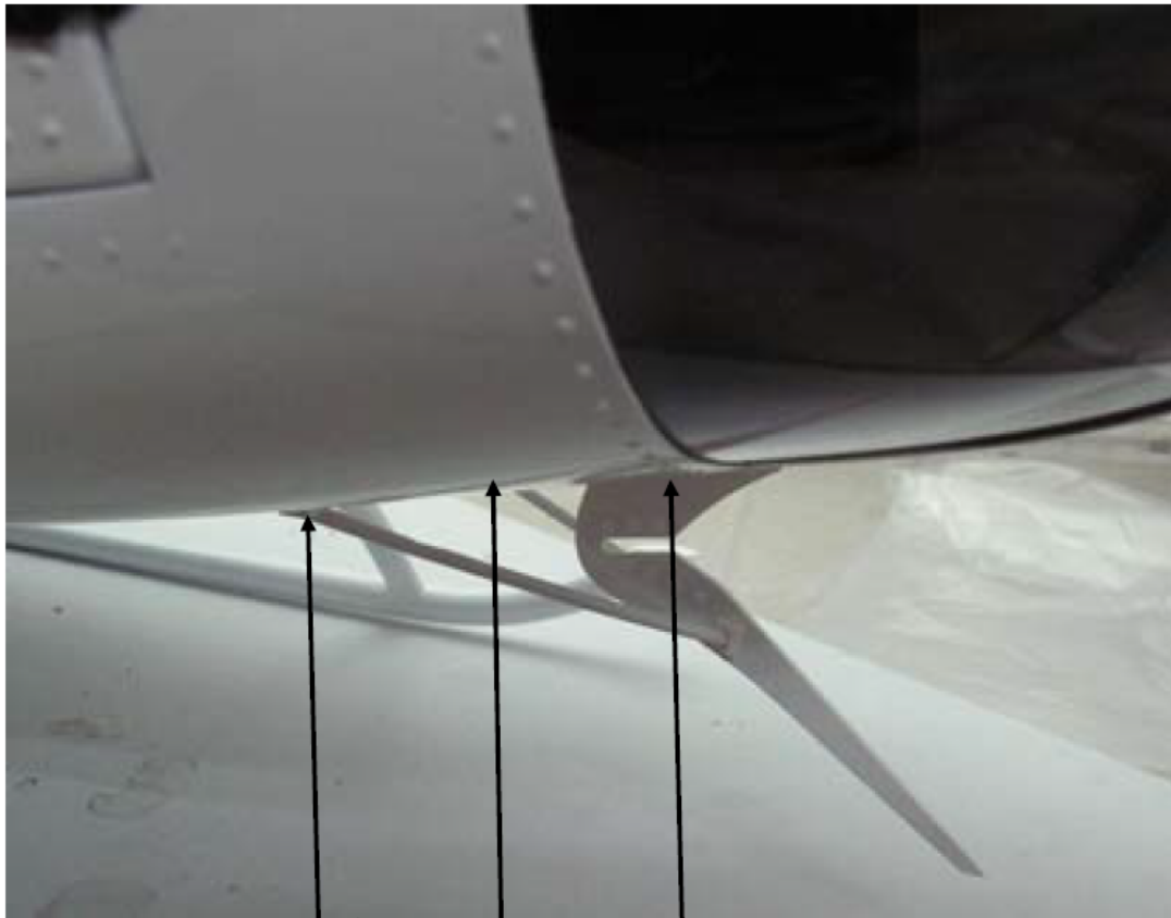
Glue the lower wire cutter and supports (48) + (49) into position as shown.
