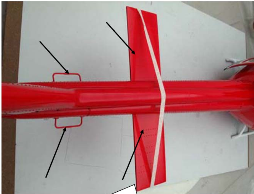
Glue tail fins and aerals (43) + (47) into position as shown. Use tape to secure them while the glue cures.
