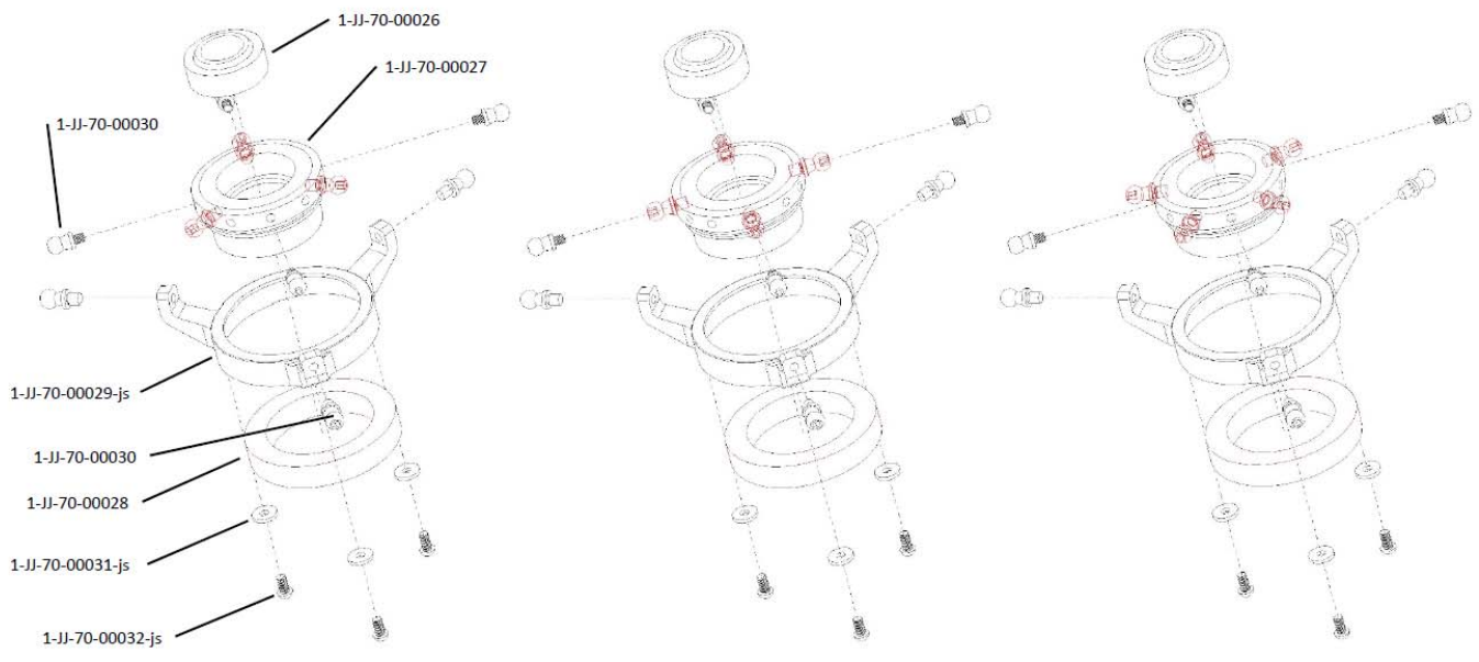
3 blade swash plate
