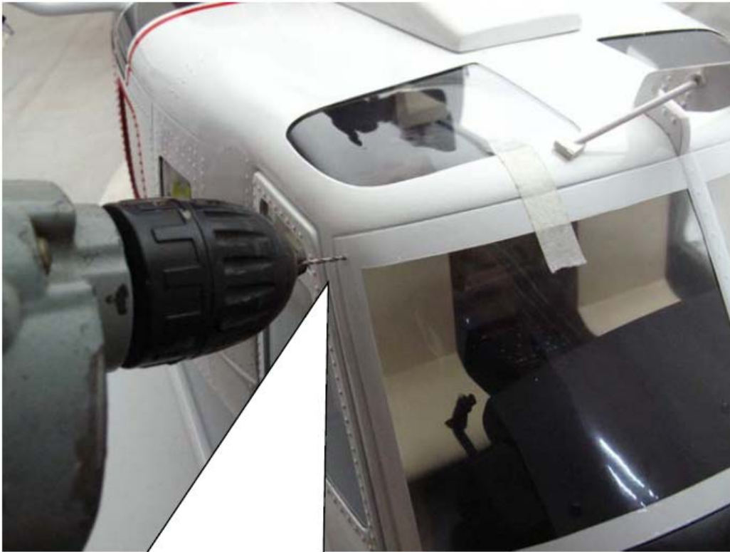
Allocate the front window properly with tape and drill four 1.5mm through holes in each corner.
