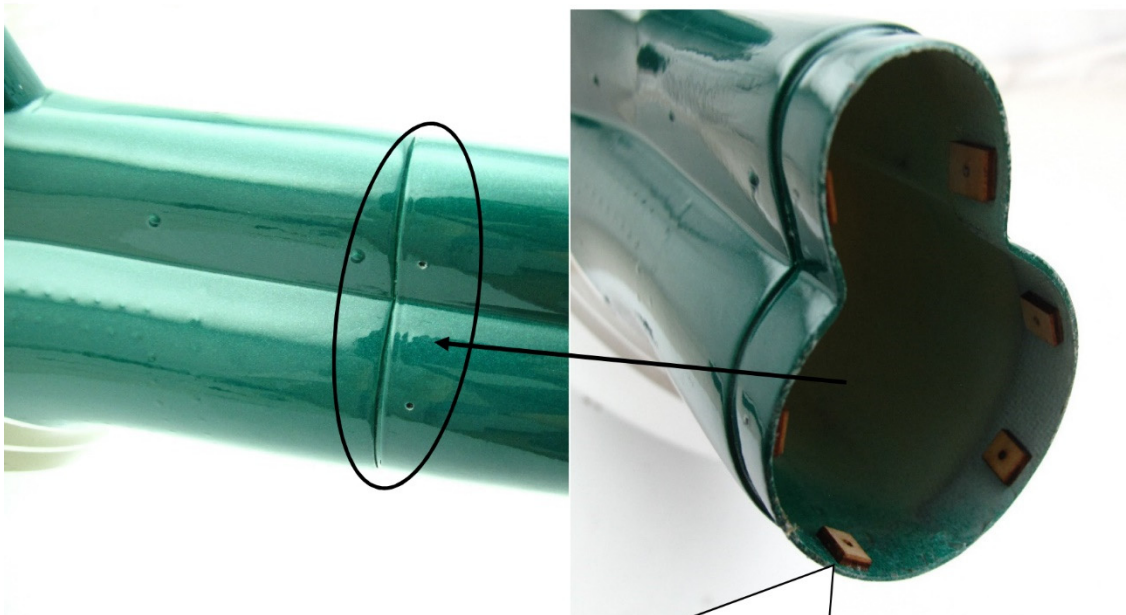
Align the tail boom properly and drill 6 holes through as shown. Glue the wooden washers 【33】 from the inside into the tail boom.
